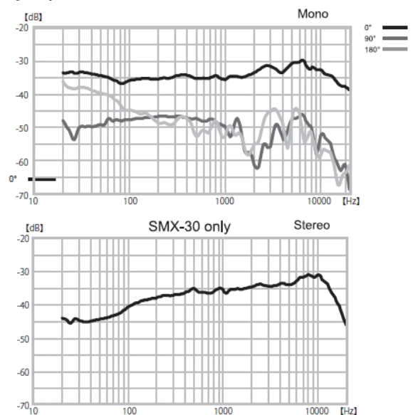
Frequency Response: Mono / Stereo
